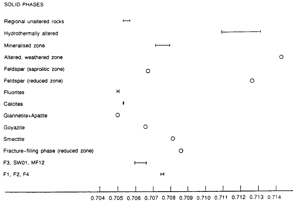
Figure 15. Strontium isotope data. Values along the bottom are ^{87}\text{Sr}/^{86}\text{Sr} isotope ratios.
