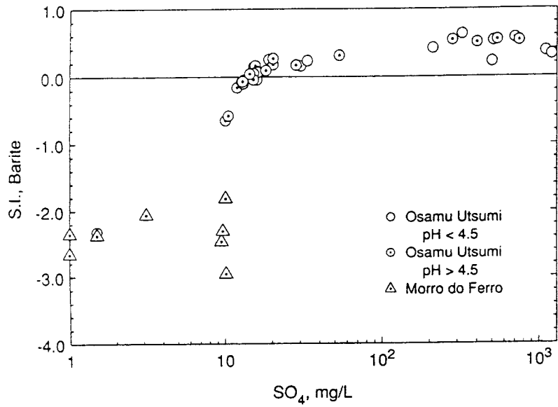
Figure 9. Barite saturation indices plotted against sulphate concentrations demonstrating stoichiometric solubility control but at a consistent level of supersaturation.
