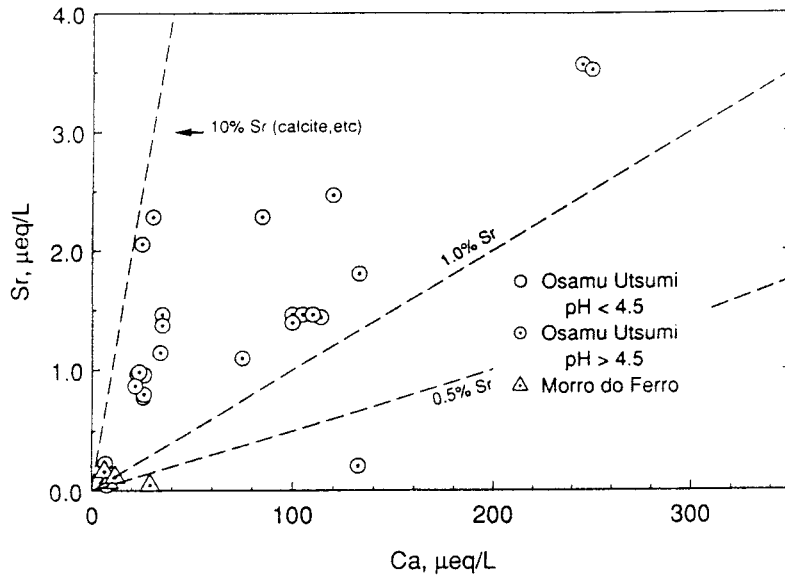
Figure 13. Strontium concentrations plotted against calcium concentrations for the dilute waters.
